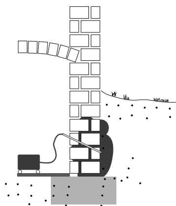
Injection de surface
